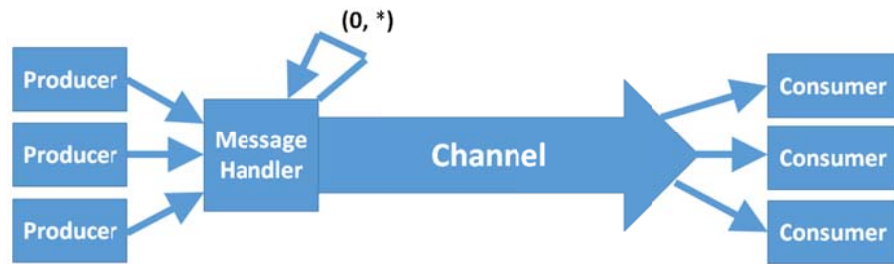
Figure 6. TAXII 2.0 proposed channel architecture [i.5]
