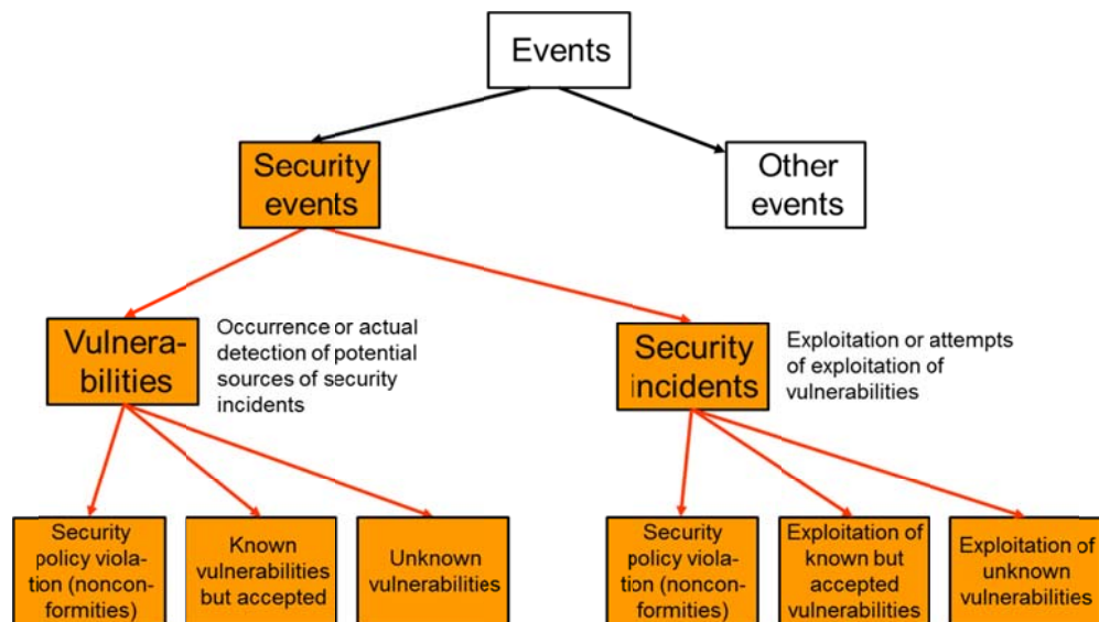
Figure 8: Relationships between different kinds of events [i.11]
