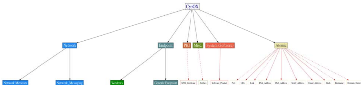
Figure 7. CybOX 2.1.1 objects and relationships [i.4]
