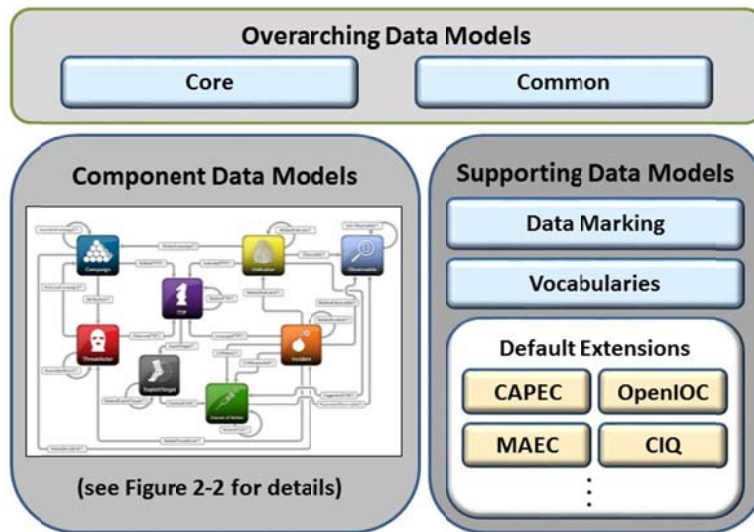
Figure 3: STIX architecture [i.4]
