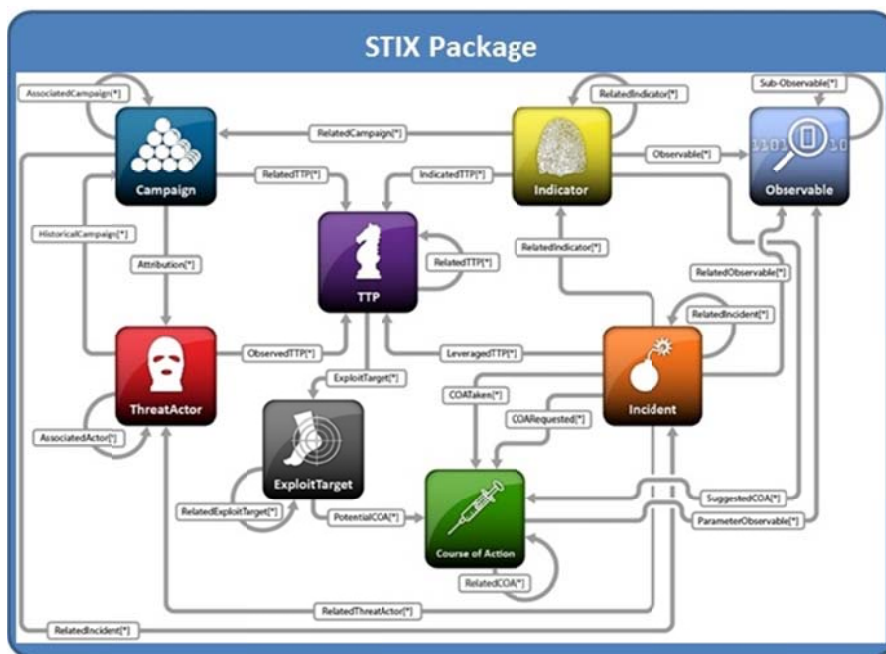
Figure 2: STIX Package encompasses the STIX individual component data models [i.4]
