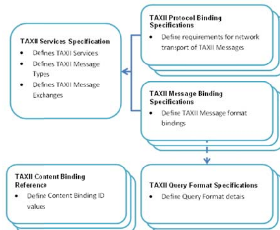
Figure 5. TAXII specification components [i.4]
