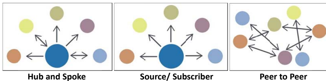
Figure 4. TAXII models supported [i.4]
