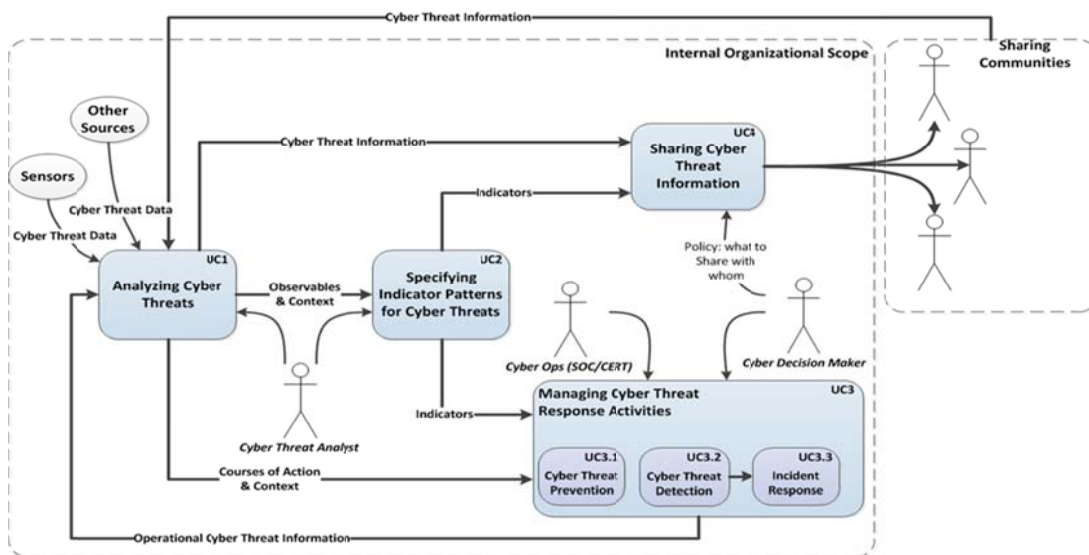
Figure 1: STIX use cases [i.4]
