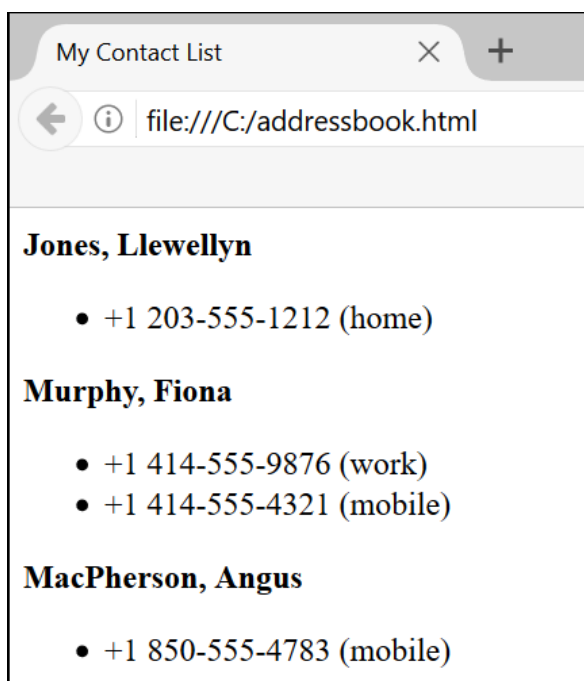
Figure 4: addressbook.html
