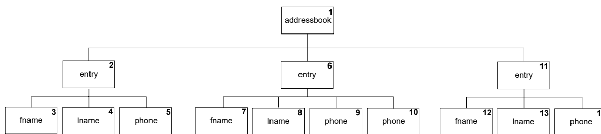
Figure 2: addressbook.xml tree
