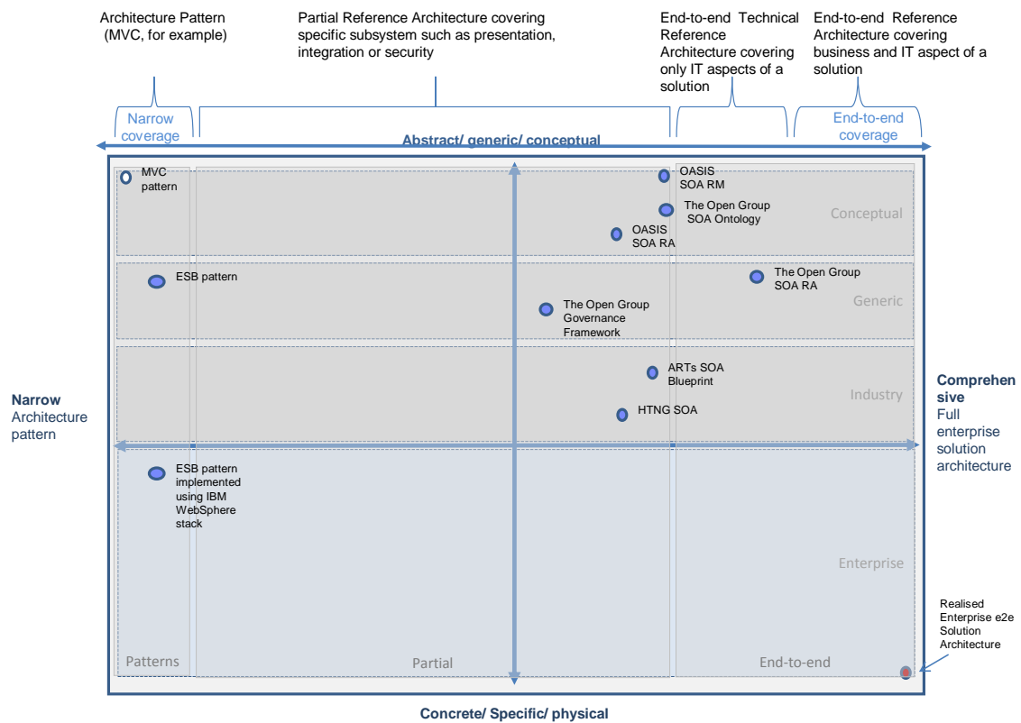
Figure 21: SOA Standards
