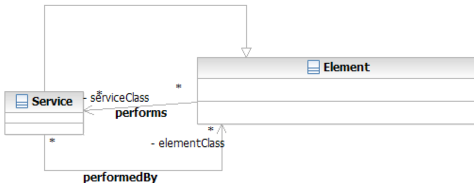
Figure 8: The Service Class
