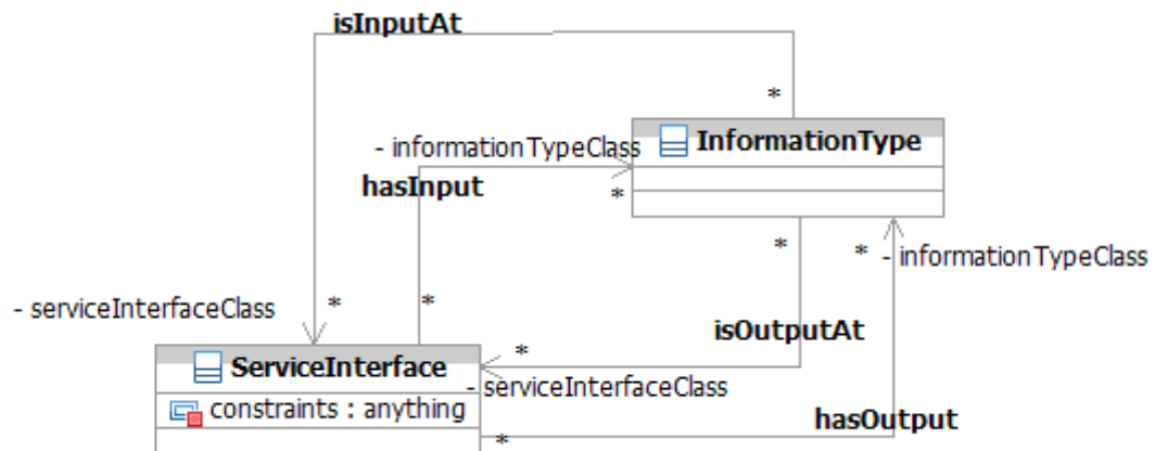
Figure 12: The InformationType Class
